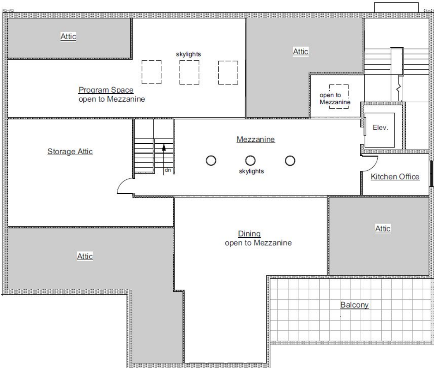
Mezzanine Plan
